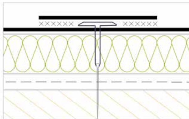
FIG. 7 MECHANICAL FASTENING – FIELD FASTENING OF MEMBRANE
