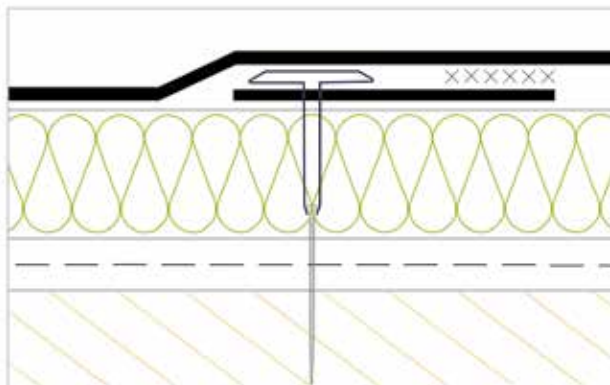
FIG.9 MECHANICAL FASTENING: SECRET FIX FASTENING OF MEMBRANE
